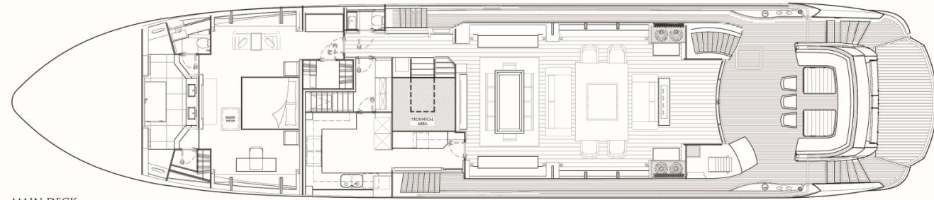
MAIN DECK
