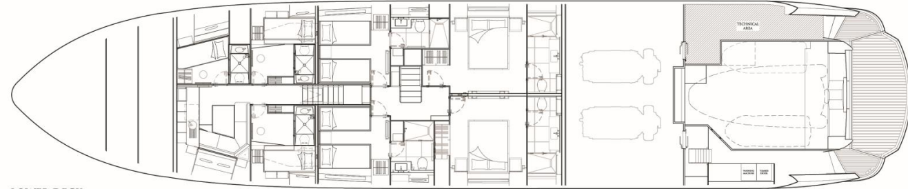
LOWER DECK
